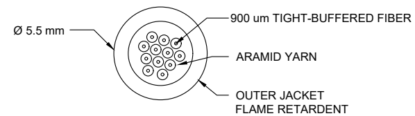
VIEW A CROSS SECTION NOT TO SCALE
