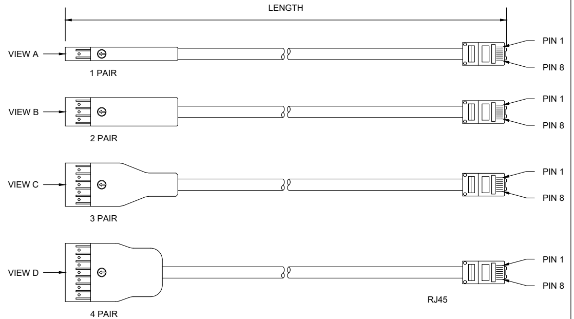
110 CONNECTOR FOR CAT 6 DEPICTED
