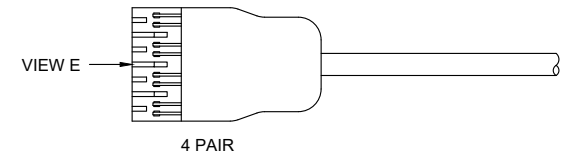
110 CONNECTOR FOR CAT 6 DEPICTED
