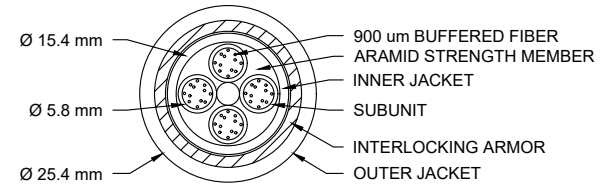
VIEW A CROSS SECTION NOT TO SCALE
