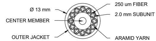
VIEW A CROSS SECTION NOT TO SCALE
